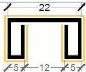
GLASS RAILING TOP DL-22
