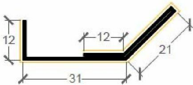
SHUTTER HANDLE DL-32
